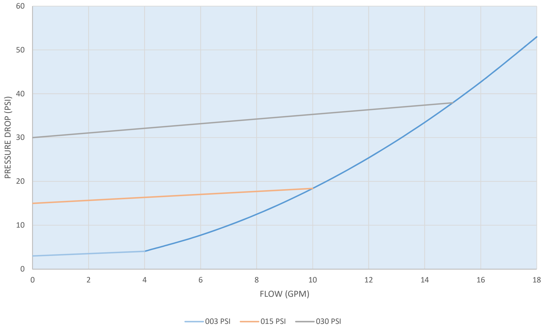
ICT-B-10 FLOW VERSUS PRESSURE DROP ISO 68 OIL, 100F
